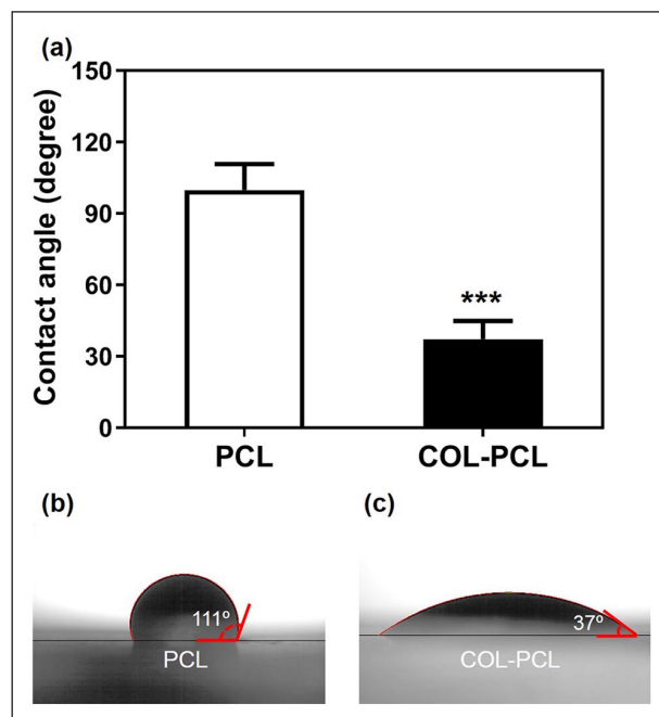
Figure 3. Water contact angle measurement of PCL and COL-PCL nanofiber membrane. Photographs of water droplet on the PCL (b) and COL-PCL (c) nanofiber membrane to measure the contact angle. The values shown are means \pm SEs ( n=3 ). * denotes statistical significance difference (***: p < 0.001 ) compared to PCL.
