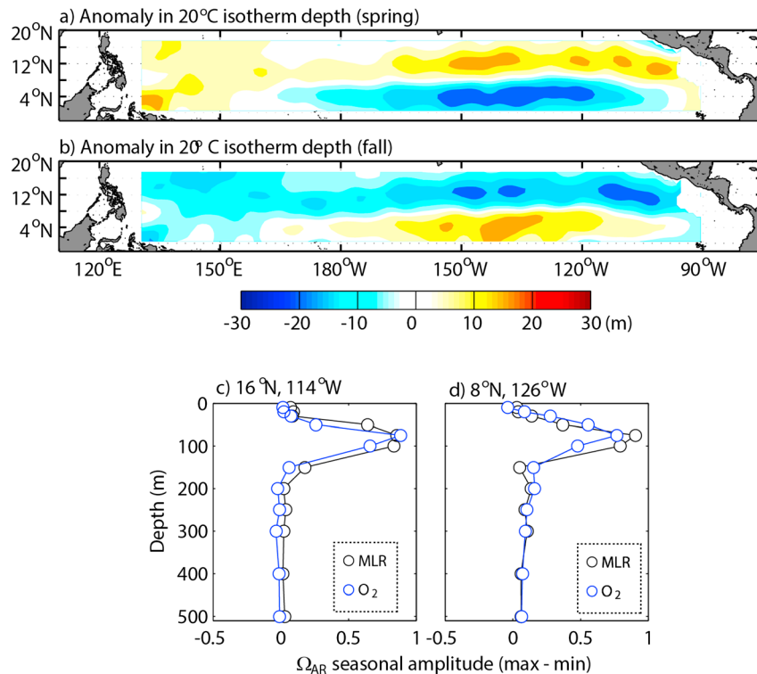
Figure 4. Anomaly in the depth of 20°C isotherm during (a) spring and (b) fall. Vertical profiles of seasonal amplitude (max – min) of \Omega_{AR} for 4^\circ \times 4^\circ areas centered at (c) 16°N, 114°W and (d) 8°N, 126°W. The black and blue symbols represent multiple linear regression (MLR)-based predictions and O_2 -based estimates, respectively. The O_2 -based estimates were obtained from the observed total alkalinity (TA) and total inorganic carbon (TIC) values [Key et al., 2004] and the amount of change in TIC expected due to seasonal amplitude of the O_2 concentration based on the ratio of Anderson and Sarmiento [1994].
