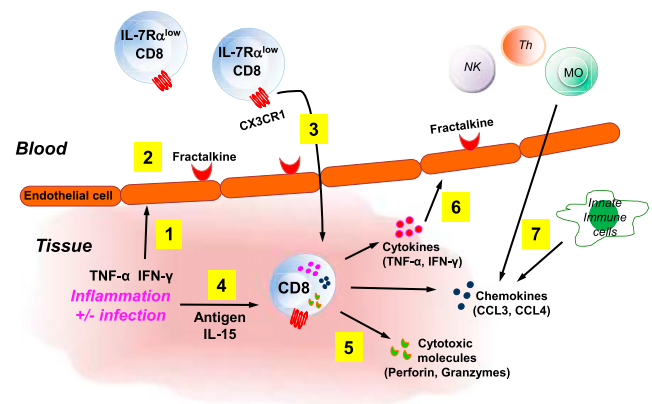
FIGURE 8. A proposed model for the role of IL-7R \alpha^{low} effector memory CD8 + T cells in promoting inflammation by forming an amplification loop of CX3CR1 and fractalkine. In response to an infection or tissue damage at a peripheral site, IFN- \gamma and TNF- \alpha are secreted from innate immune cells like NK cells and macrophages (1), leading to inducing the expression of fractalkine by endothelial cells (2). In the bloodstream, CX3CR1-expressing IL-7R \alpha^{low} EM CD8 + T cells and other immune cells (data not shown) migrate to the endothelial cells in response to fractalkine and move into the infected or damaged peripheral site (3) where activated IL-7R \alpha^{low} EM CD8 + T cells (4) promote inflammation by producing chemokines (CCL3 and CCL4), cytokines (IFN- \gamma and TNF- \alpha ), and cytotoxic molecules (perforin and granzymes) with further immune cell recruitment, activation, and tissue damage (5–7). Also, the secreted IFN- \gamma and TNF- \alpha further fractalkine expression on the endothelial cells, resulting in additional recruitment of CX3CR1-expressing IL-7R \alpha^{low} EM CD8 + T and other cells by forming an amplification loop of IL-7R \alpha^{low} EM CD8 + T cells, CX3CR1, and fractalkine that augments inflammation (6).
