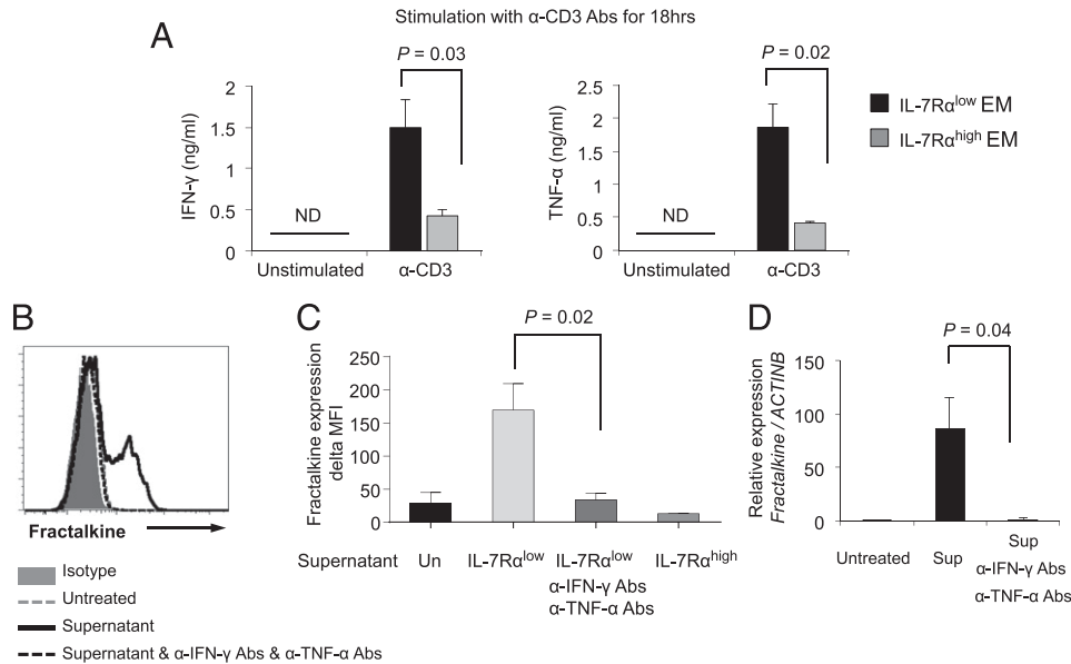
FIGURE 7. IL-7R \alpha^{low} effector memory CD8 + T cells produce high levels of IFN- \gamma and TNF- \alpha , leading to up-regulation of fractalkine expression by HUVECs. (A) ELISA of IFN- \gamma and TNF- \alpha in culture supernatants of FACS-sorted IL-7R \alpha^{low} and IL-7R \alpha^{high} EM CD8 + T cells that were incubated for 18 h with or without anti-CD3 Abs. (B–D) HUVECs were incubated for 8 h in the culture supernatants (Sup, 10% final concentration) of anti-CD3 Ab-stimulated IL-7R \alpha^{low} or IL-7R \alpha^{high} EM CD8 + T cells from (A) in the presence or absence of human anti-IFN- \gamma and -TNF- \alpha neutralizing Abs (1 \mu g/ml for both). Un, not treated with supernatant. (B and C) Flow cytometric analysis of fractalkine by HUVECs. (B) Representative histograms of the flow cytometric analysis. (C) \Delta MFI values of fractalkine expression were obtained by subtracting MFI values of isotype control staining from MFI values of fractalkine staining. (D) RT-qPCR analysis of fractalkine gene expression in HUVECs. Bars and error bars indicate the mean and SEM, respectively ( n = 3 (A) and n = 2 –5 (C and D)).
