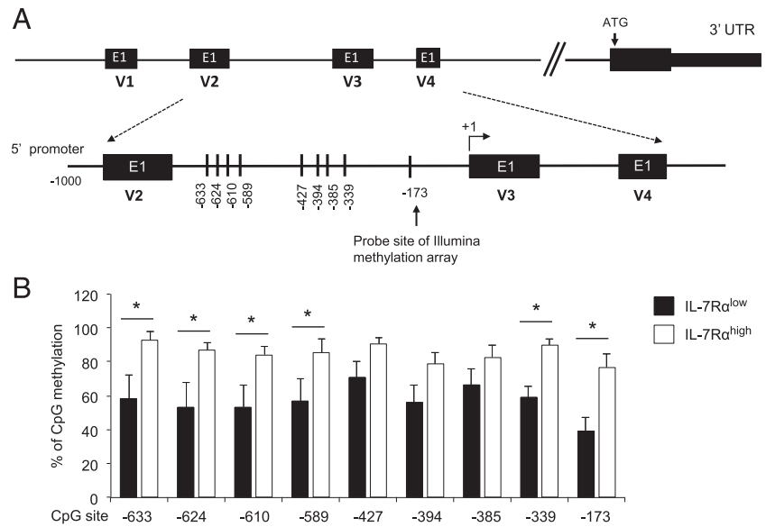
FIGURE 3. DNA methylation profiles in the CX3CR1 gene promoter are different in IL-7R \alpha low and IL-7R \alpha high effector memory CD8 + T cells. (A) Illustration of the promoter regions of four CX3CR1 transcript variants (V1, V2, V3, and V4) and detailed map of analyzed CpG sites. The first exons (E1) of individual variants are indicated in black boxes. The CpG site (-173) included in the original DNA methylation array chip and additional CpG sites (0 to -1 KB) are indicated with vertical lines and numbers. The latter numbers were given in respect to the first nucleotide of the first exon of variant 3 (+1). (B) Methylation status of CpG sites in the CX3CR1 gene promoter region depicted in (A) among IL-7R \alpha low and IL-7R \alpha high EM CD8 + T cells. Details for bisulfite treatment and DNA methylation analysis are stated in Materials and Methods . Bars and error bars indicate the mean and SEM for individual CpG sites in IL-7R \alpha low and IL-7R \alpha high EM CD8 + T cells, respectively ( n = 7 donors). * p < 0.05 .
