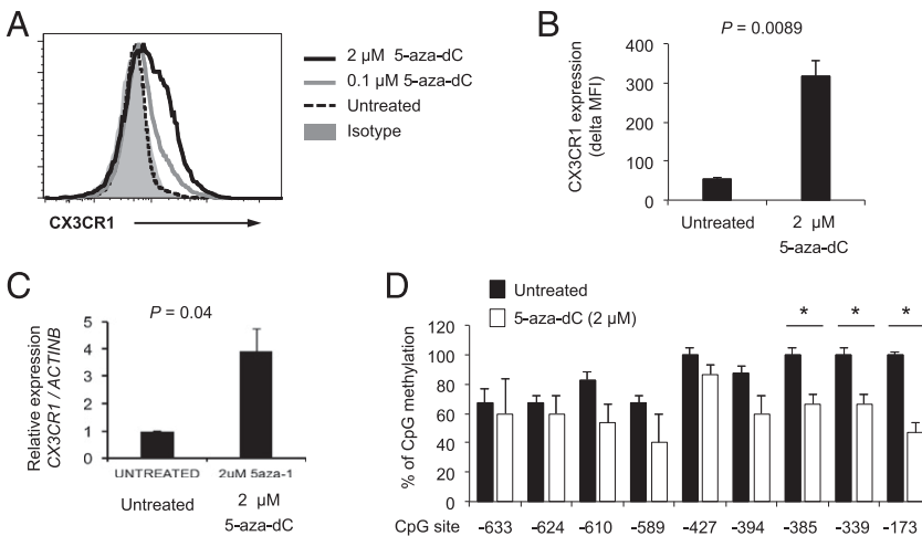
FIGURE 4. 5-aza-dC upregulates the expression of CX3CR1 by Jurkat T cells. Jurkat T cells were cultured for 4 d with or without 5-aza-dC (0, 0.1, and 2 \mu M). (A) and (B) Flow cytometric analysis of CX3CR1 expression on untreated and 5-aza-dC-treated Jurkat T cells. (A) Representative histograms of CX3CR1 and isotype control staining. (B) \Delta MFI of CX3CR1 expression obtained by subtracting MFI values of isotype controls from MFI values of CX3CR1 staining. (C) RT-qPCR analysis of CX3CR1 gene expression in untreated and 5-aza-dC-treated Jurkat T cells. (D) The methylation status of individual CpG sites in the CX3CR1 gene promoter in untreated and 5-aza-dC-treated Jurkat T cells at day 4. Bars and error bars indicate the mean and SEM, respectively [ n = 3 (B), n = 7 (C), and n = 3 (D)]. * p < 0.05 .
