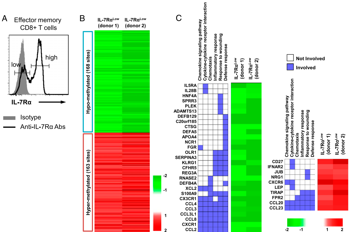
FIGURE 1. Human IL-7R\alpha^{low} and IL-7R\alpha^{high} effector memory CD8 + T cells have differential DNA methylation. IL-7R\alpha^{low} and IL-7R\alpha^{high} EM (CCR7 - ) CD8 + T cells were purified from fresh PBMCs of two healthy donors using a FACSaria. DNA were purified from sorted cells and analyzed using an Illumina human DNA methylation array chip (see details in Materials and Methods ). (A) Representative histograms showing IL-7R\alpha^{low} and IL-7R\alpha^{high} cells in human peripheral EM CD8 + T cells. (B) Heat map showing the pattern of differentially methylated CpG sites between IL-7R\alpha^{low} and IL-7R\alpha^{high} EM CD8 + T cells. The red and green colors indicate increased and decreased methylation of CpG sites, respectively. (C) The most significantly enriched annotation cluster by the genes with differentially methylated sites in IL-7R\alpha^{low} and IL-7R\alpha^{high} EM CD8 + T cells. Two-dimensional map displays the genes that are involved in the annotation cluster. Heat map display the representative differential methylation patterns of the genes in IL-7R\alpha^{low} EM CD8 + T cells compared with IL-7R\alpha^{high} EM CD8 + T cells. Left and right panels are for the genes with decreased and increased methylation, respectively.
