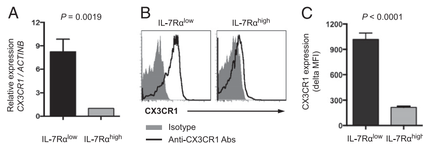
FIGURE 2. Human IL-7R \alpha low and IL-7R \alpha high effector memory CD8 + T cells have different levels of CX3CR1 gene and protein expression. (A) RT-qPCR analysis of CX3CR1 gene expression in FACS-sorted IL-7R \alpha low and IL-7R \alpha high EM CD8 + T cells of healthy individuals ( n=5 ). (B and C) Flow cytometric analysis of CX3CR1 expression on IL-7R \alpha low and IL-7R \alpha high EM CD8 + T cells in peripheral blood of healthy people ( n=39 ). (B) Representative histograms of CX3CR1 and isotype control staining. (C) Mean fluorescence intensity (MFI) of CX3CR1 expression by IL-7R \alpha low and IL-7R \alpha high EM CD8 + T cells. \Delta MFI of CX3CR1 expression was obtained by subtracting MFI of isotype control staining from MFI of CX3CR1 staining. Bars and error bars indicate mean and SEM, respectively.
