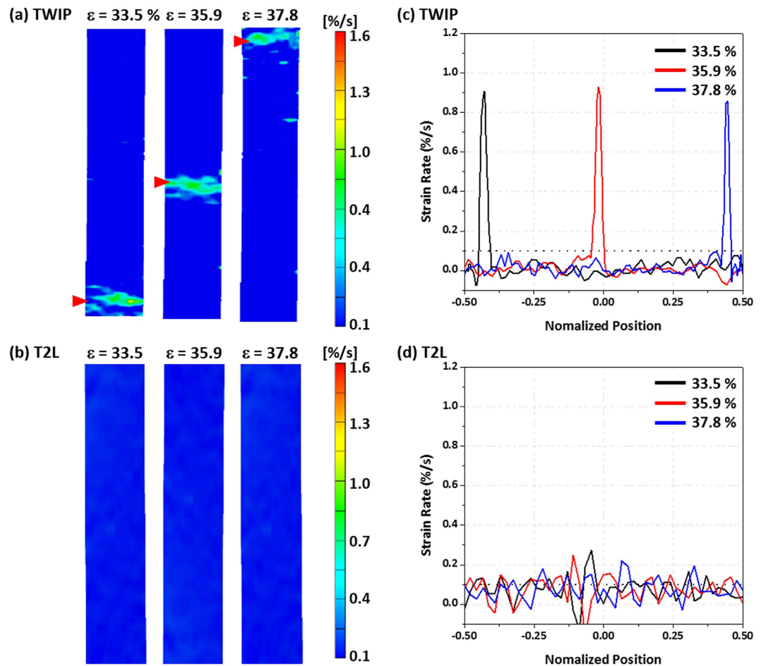
Figure 5. (a,b) Digital images of strain rate and (c,d) strain rate distribution curves of the TWIP and T2L sheets at tensile strains of 33.5%, 35.9%, and 37.8%. In the TWIP sheet, the localization of strain rate occurs in a form of band at the lower region of the gage section at the strain of 33.5%. This localized band moves upward as the strain increases to 35.9% and 37.8%. In the T2L sheet, the localized band is not found throughout the gage section, and the strain rate is almost same to the overall strain rate (0.1%/s) of the tensile test.
