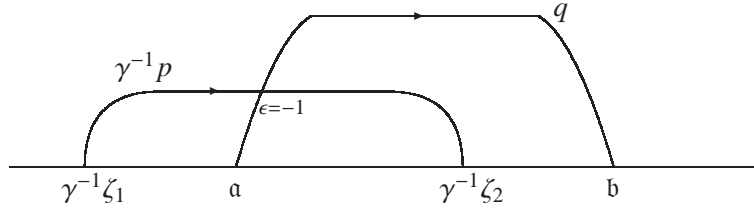
FIGURE 24. Illustration of case a \in (\gamma^{-1}\zeta_1, \gamma^{-1}\zeta_2)_{cycl} and b \in (\gamma^{-1}\zeta_2, \gamma^{-1}\zeta_1)_{cycl} in Table 5. The path \gamma^{-1}p crosses q from left to right.
