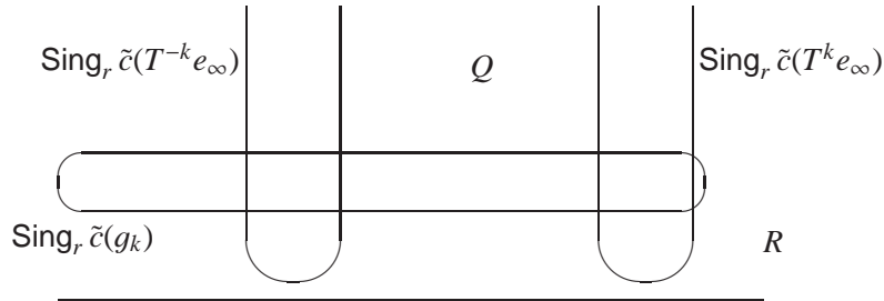
FIGURE 20. Illustration of regions of non-holomorphy.
