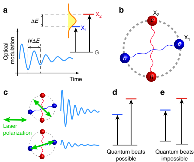
Fig. 1 Quantum beats in \text{ReS}_2 . a Coherent superposition of resonantly excited two excitons (blue ( X_1 ) and red ( X_2 ) states) can lead to beating optical signals in the time domain (light blue oscillation). The oscillation period corresponds exactly to the energy difference ( \Delta E ) of the excited states. b Illustration of anisotropic excitons (dumbbell-shaped electron-hole pairs) in \text{ReS}_2 . The two lowest excitons, X_1 and X_2 , are linearly polarized with different in-plane orientations. c Controlling quantum beats (light blue oscillations) of excitons by manipulating laser polarization (arrows). Blue (red) color represents X_1 ( X_2 ). While the quantum beat is expected to be large when optical polarization is adjusted to excite both two excitons in a balanced way (upper schematics), it will weaken if only one of the two exciton states is excited by light asymmetrically (lower schematics). d, e Three-level system with a common state ( d ) and two independent two-level systems ( e )
