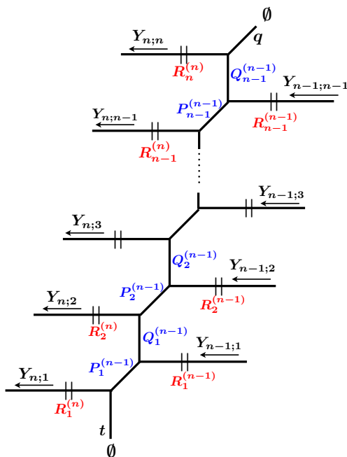
Figure 26. The component diagram which gives the factor A_n(\vec{Y}_n, \vec{Y}_{n-1}) .
