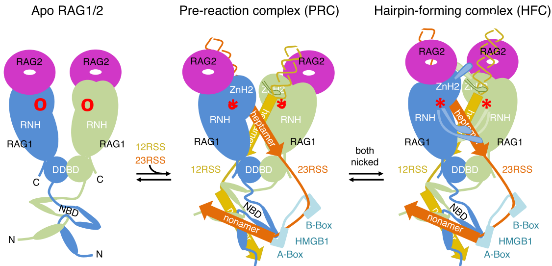
Figure 7. Cartoon Diagrams of the Reaction Process of RAG1/2 from the Apo Form to the PRC and the HFC
