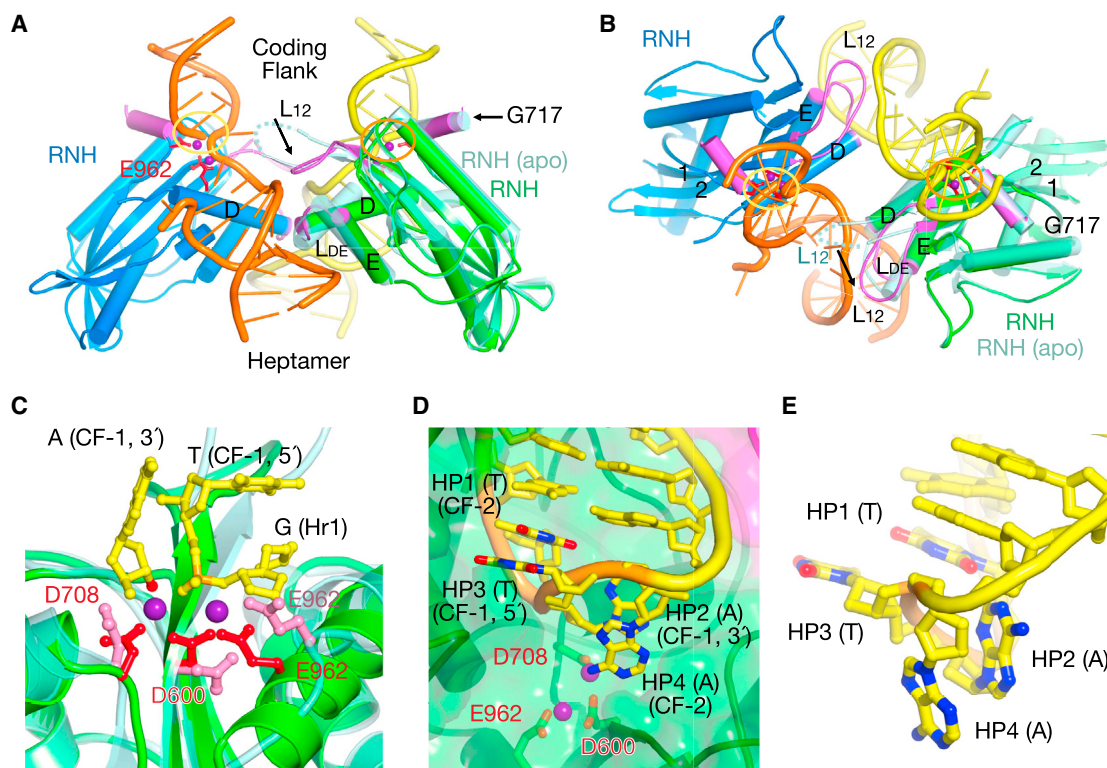
Figure 6. The Active Site and Hairpin Formation
