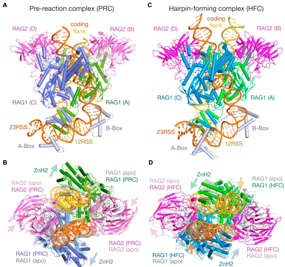
Figure 1. Structures of RAG1/2 PRC and HFC with 12/23-RSS DNAs
