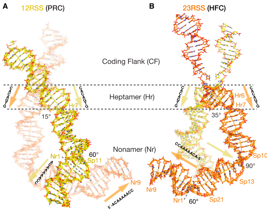
Figure 3. The Overall Curvature of 12/23-RSS DNAs
